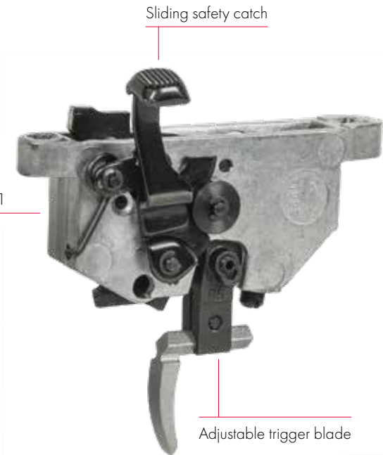
Two stage trigger 5098/71
